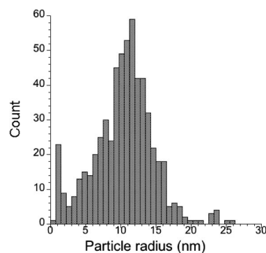
Figure 2. Top: TEM field-view image at 10000 \times of nano- 9 . The inset shows a detail at 50000 \times . Bottom: Histogram of particle count as a function of particle radius (nm) in the image.
